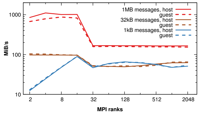
Figure 4: Parallel transfer benchmark sendrecv shows no systematic performance penalty at the 1 kB and 32 kB message sizes. At the 1 MB message size, the cost is roughly 5% once the problem grows to multiple nodes; we suspect this is due to tuning differences rather than containers.
