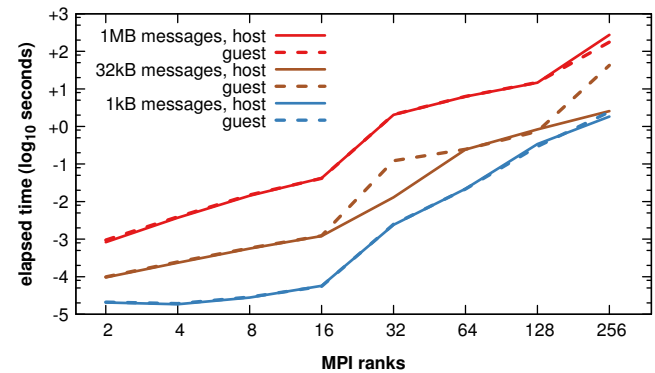
Figure 5: Collective benchmark alltoall shows no systematic performance penalty. (We suspect the glitches at 32 kB for 32 and 256 ranks, as well as 1 MB/256, are due to network, not container, issues.)
